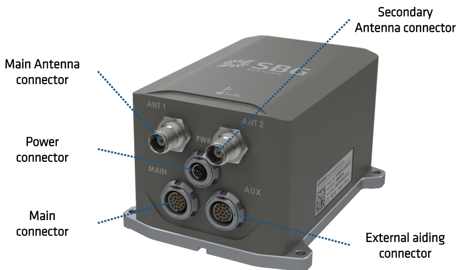
Figure 4.2: Apogee-D connectors
