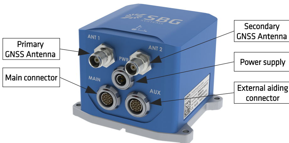
Figure 4.2: Ekinox INS with integrated GNSS receiver
