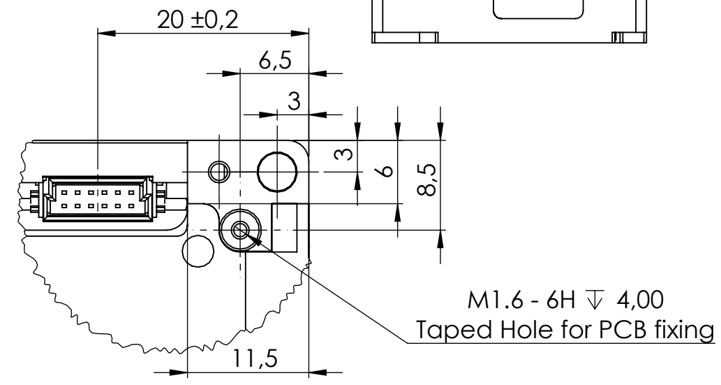
DETAIL N SCALE 2 : 1
