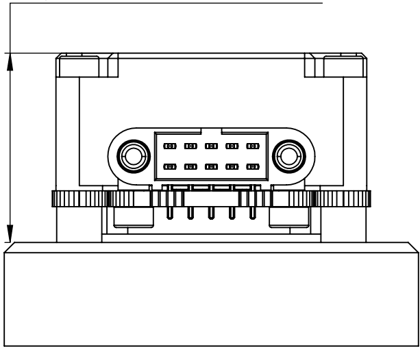
18,3 OVERALL DIMENSION
